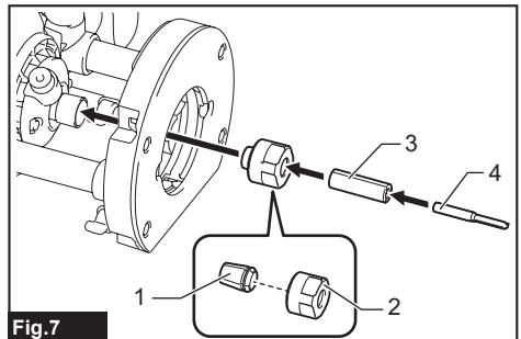
Fig. 7 ► 1. Collet cone 2. Collet nut 3. Collet sleeve 4. Router bit
