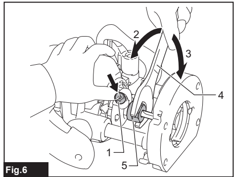
Fig. 6 ► 1. Shaft lock 2. Loosen 3. Tighten 4. Wrench 5. Collet nut
